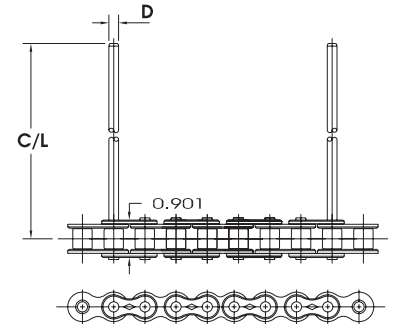
STANDARD PIN OVEN CHAIN 标准制罐运输链
