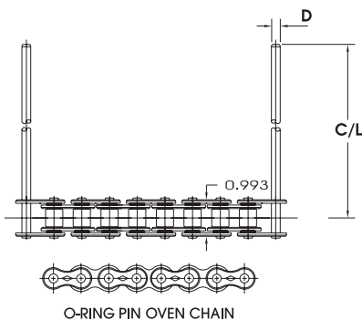
O-RING PIN OVEN CHAIN
