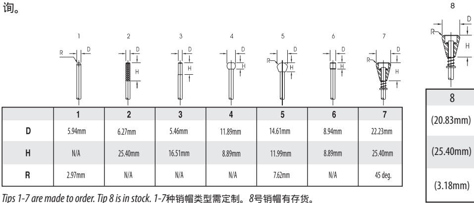
Tips 1-7 are made to order. Tip 8 is in stock. 1-7种销帽类型需定制。8号销帽有存货。
